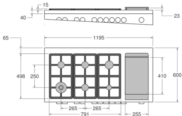
WORKTOP DETAILS
