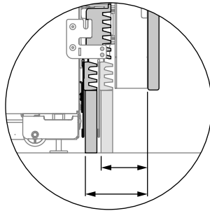
73-102mm toe kick depth measured from from rear of door panel
