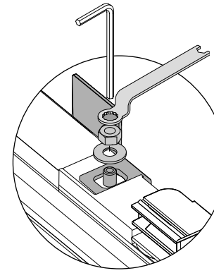
⑤ Loosely screw M8 washer and nut to adjustment screw.
