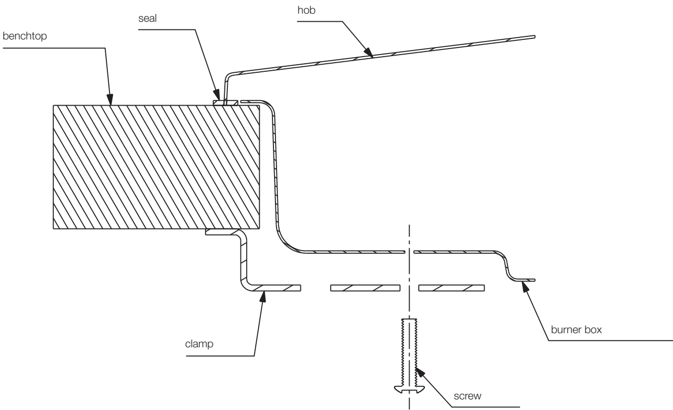
Figure 8 – Clamp fitment
