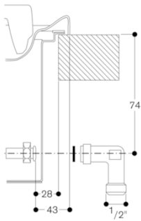
Gas connection
