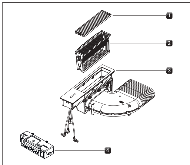
Fig. 4.5 BORA Classic cooktop extractor CKA2
