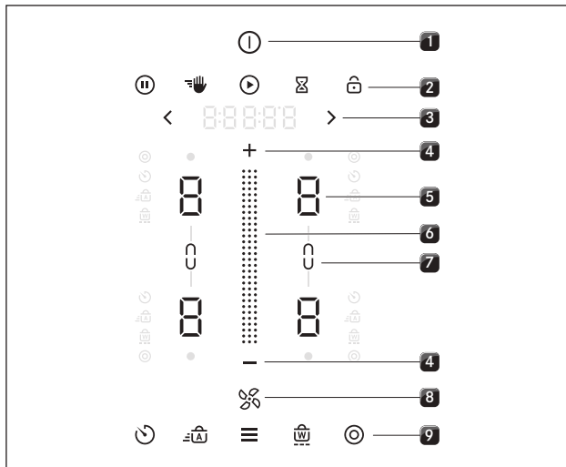
Fig. 4.2 Touch zones
