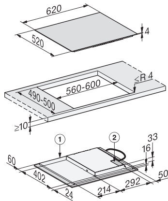
KM7220FL surface-mounted – AU (Installation drawing)
