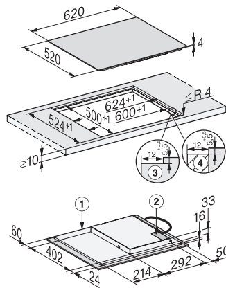
KM7220FL flush – AU (Installation drawing)
