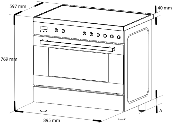
↑ Installation Details
