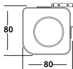
Casing Dimensions
