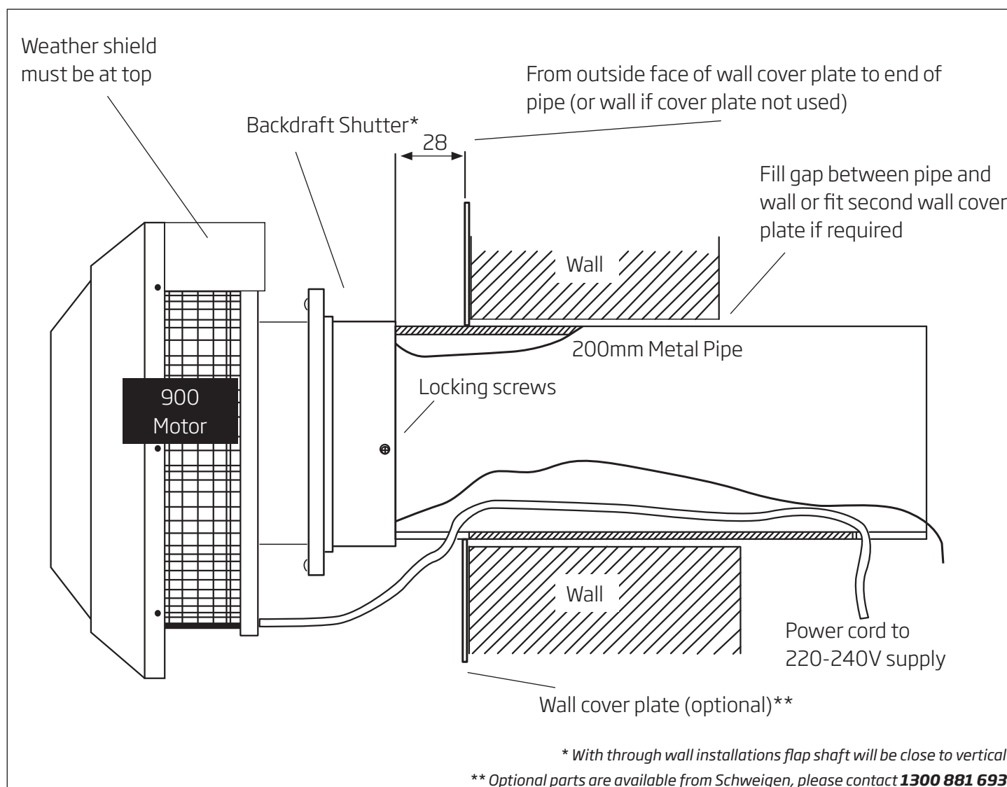
Figure 2: Wall installation
