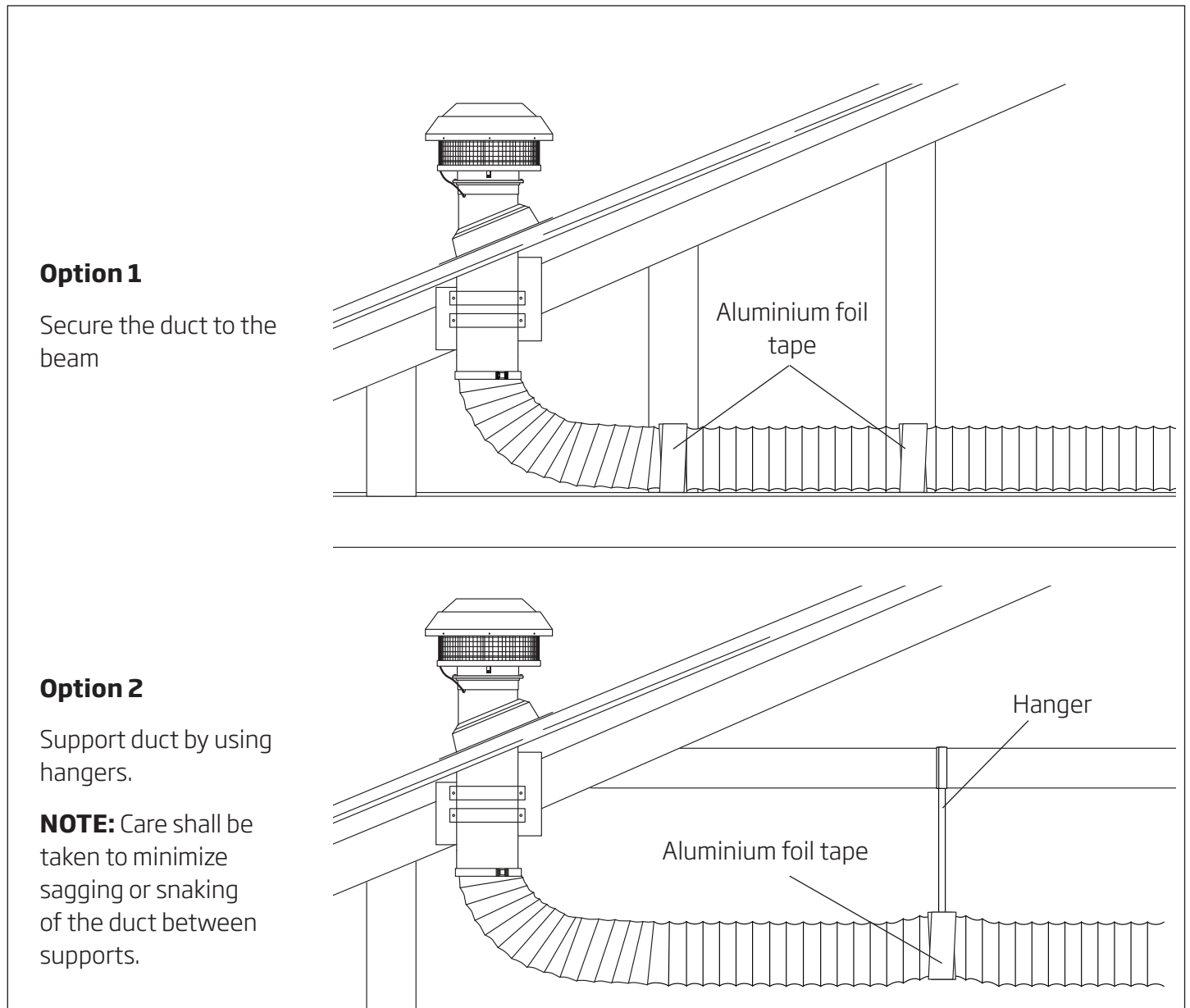
Figure 8: Securing SteelFlex™ Safety Duct
